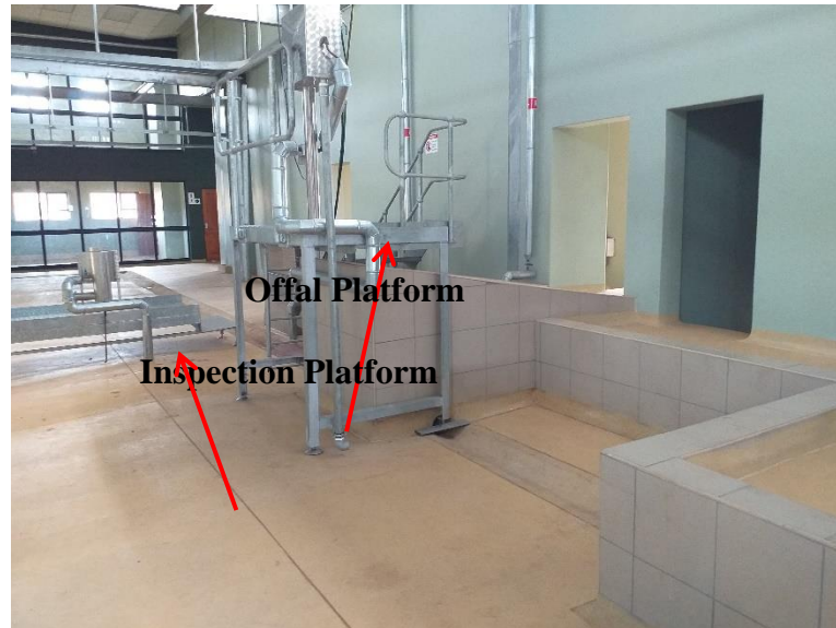
Figure 4: Offal and Inspection Platforms
